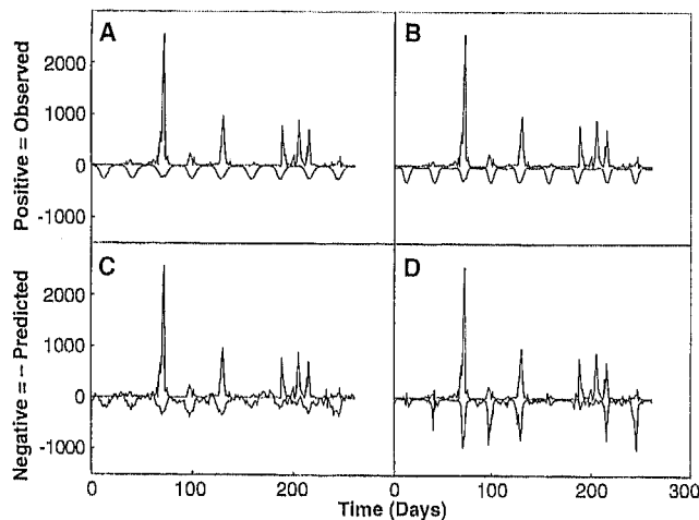
Fig. 2. Predicted versus observed values for four physical models considered (Table 1). Positive axis gives observed larval number; negative axis is (-1 \times \text{predicted value}) . (A) Linear, univariate model using lunar phase with optimal lag 19 days. (B) As in (A), but with a nonlinear model operating on lunar phase. (C) Linear, trivariate model. (D) As in (C), but with a nonlinear model. In addition to superior prediction statistics, the nonlinear trivariate model (D) best captures the erratic appearance of the series.
