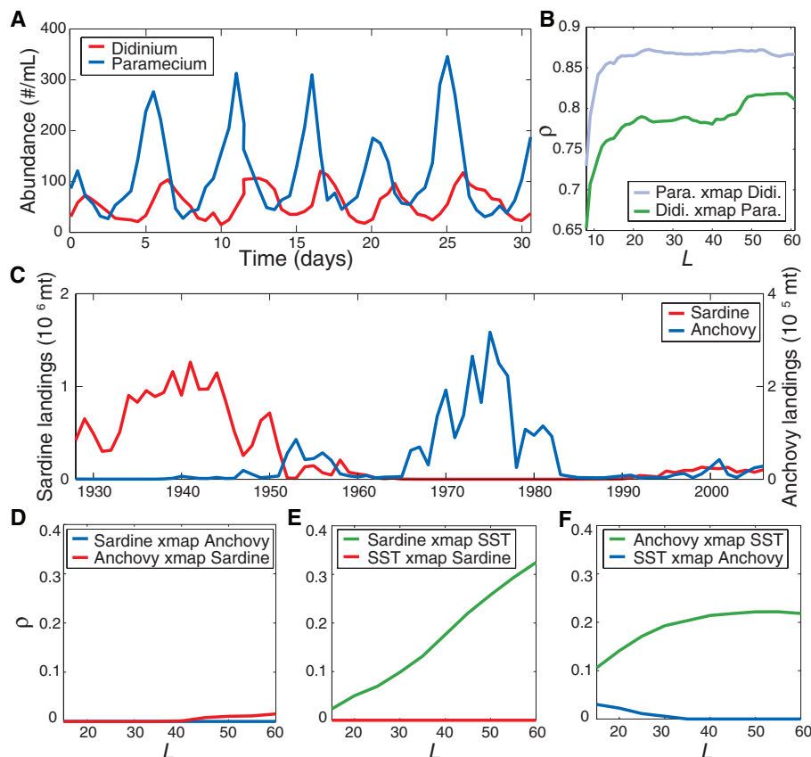
Fig. 5. Detecting causation in real time series. (A) Abundance time series of Parametium aurelia and Didinium nasutum as reported in (28). (B) CCM of Parametium and Didinium with increasing time-series length L . The pattern suggests top-down predator control. (C) California landings of Pacific sardine ( Sardinops sagax ) and northern anchovy ( Engraulis mordax ). (D–F) CCM (or lack thereof) of sardine versus anchovy, sardine versus SST (Scripps Pier), and anchovy versus SST (Newport Pier), respectively. This shows that sardines and anchovies do not interact with each other and that both are forced by temperature.
